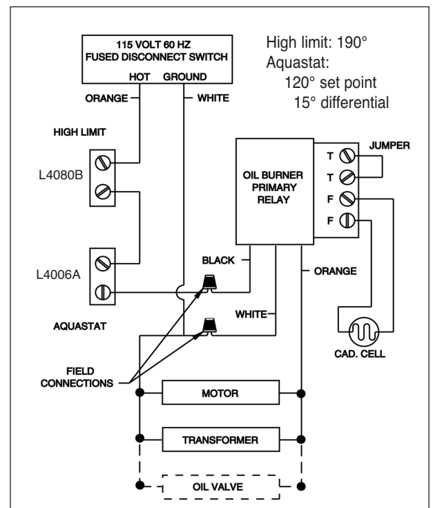
FIGURE 7: Honeywell L4006A w/ L8080B For Models: 50, 120E
