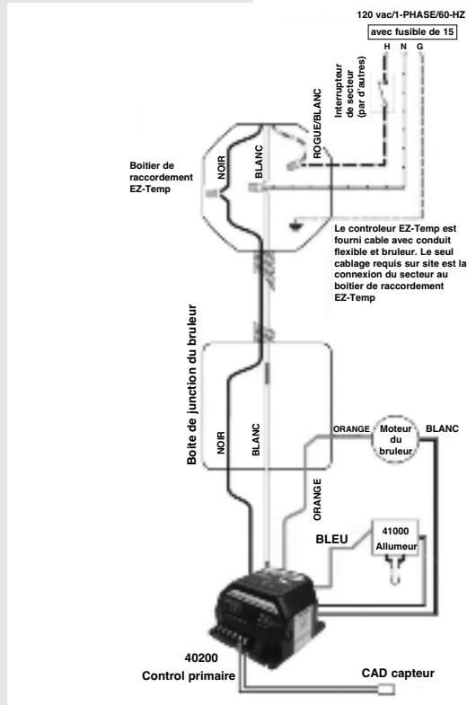
FIGURE 6 : Honeywell L4103A-1142
