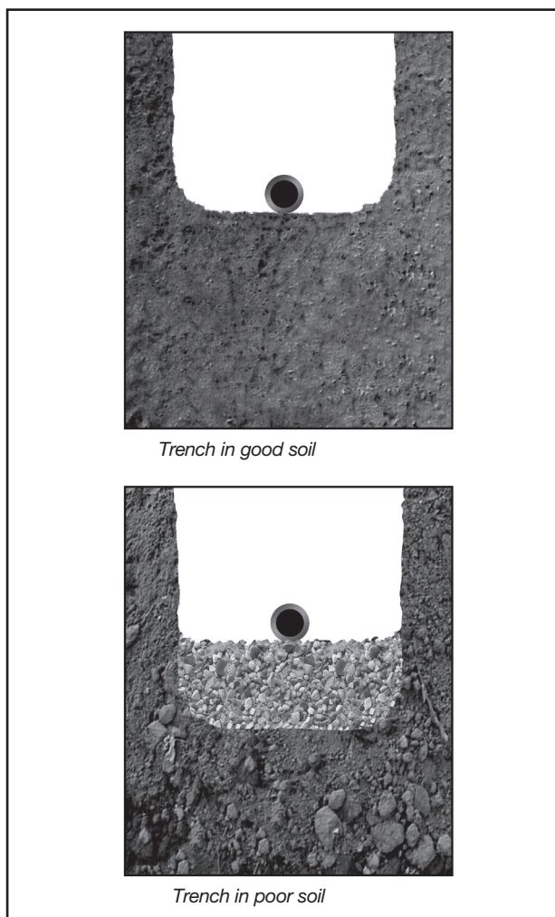
Figure 9.9 Installing PEX below grade
