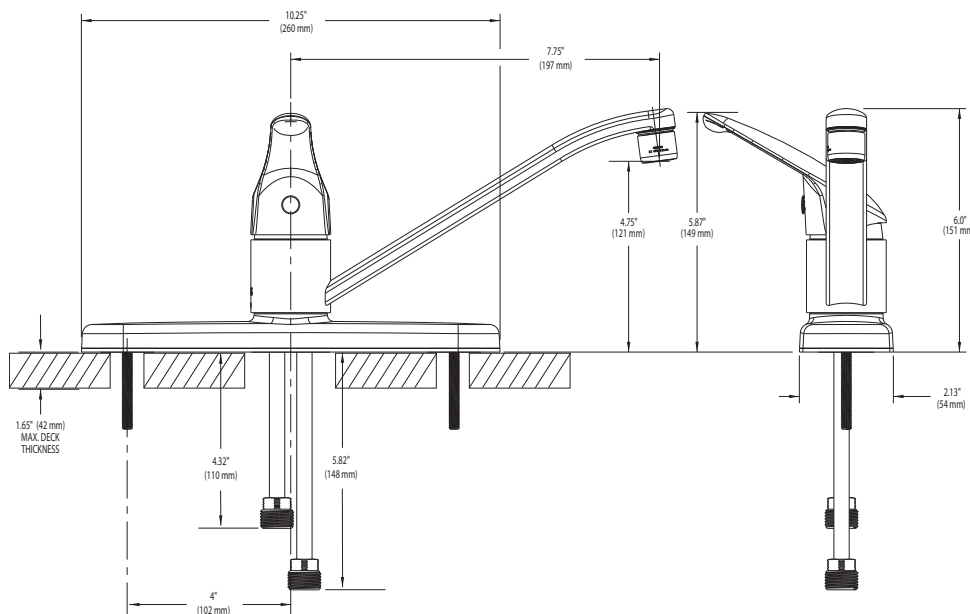
CRITICAL DIMENSIONS
