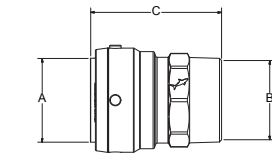
Male Connector
