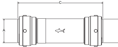
Slip Coupling
