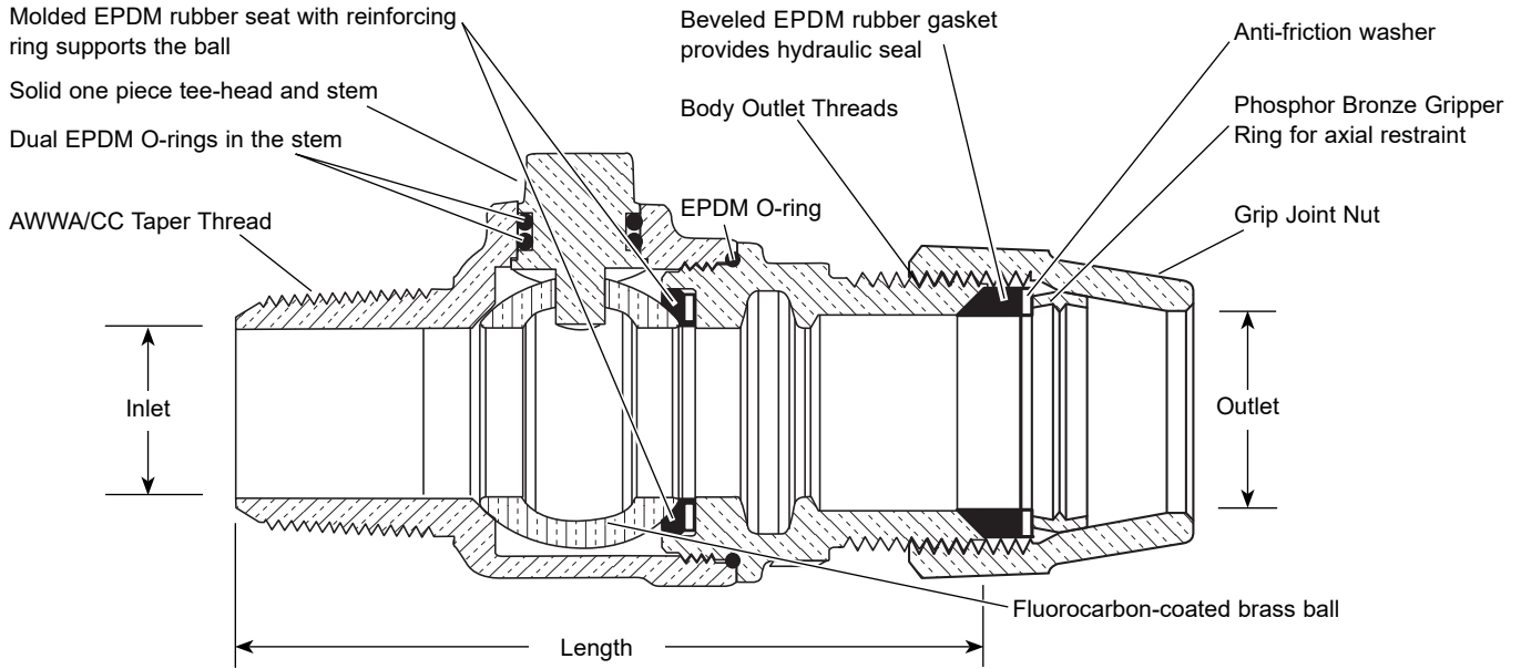
Image shown above is an FB1000-4-G-NL.
