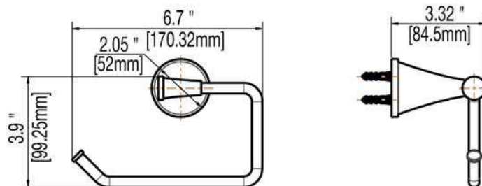
Towel Ring
