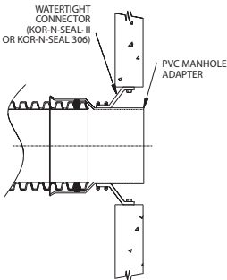
TYPE 3 WATERTIGHT USING PVC MANHOLE ADAPTER
