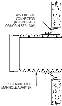
TYPE 1 WATERTIGHT USING PRE-FABRICATED ADAPTER
