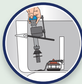
Install.
