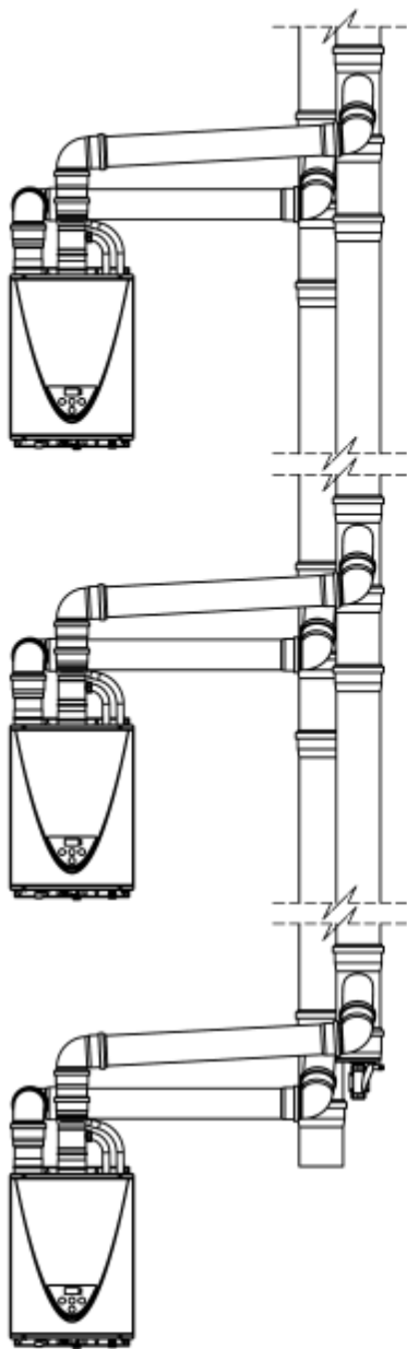
Figure 9. Vertical Venting In A Single Chase
