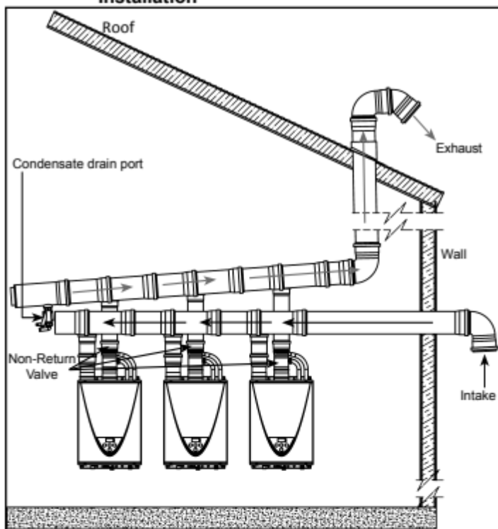
Figure 6. Typical Common-Vent Combination Wall / Roof Installation
