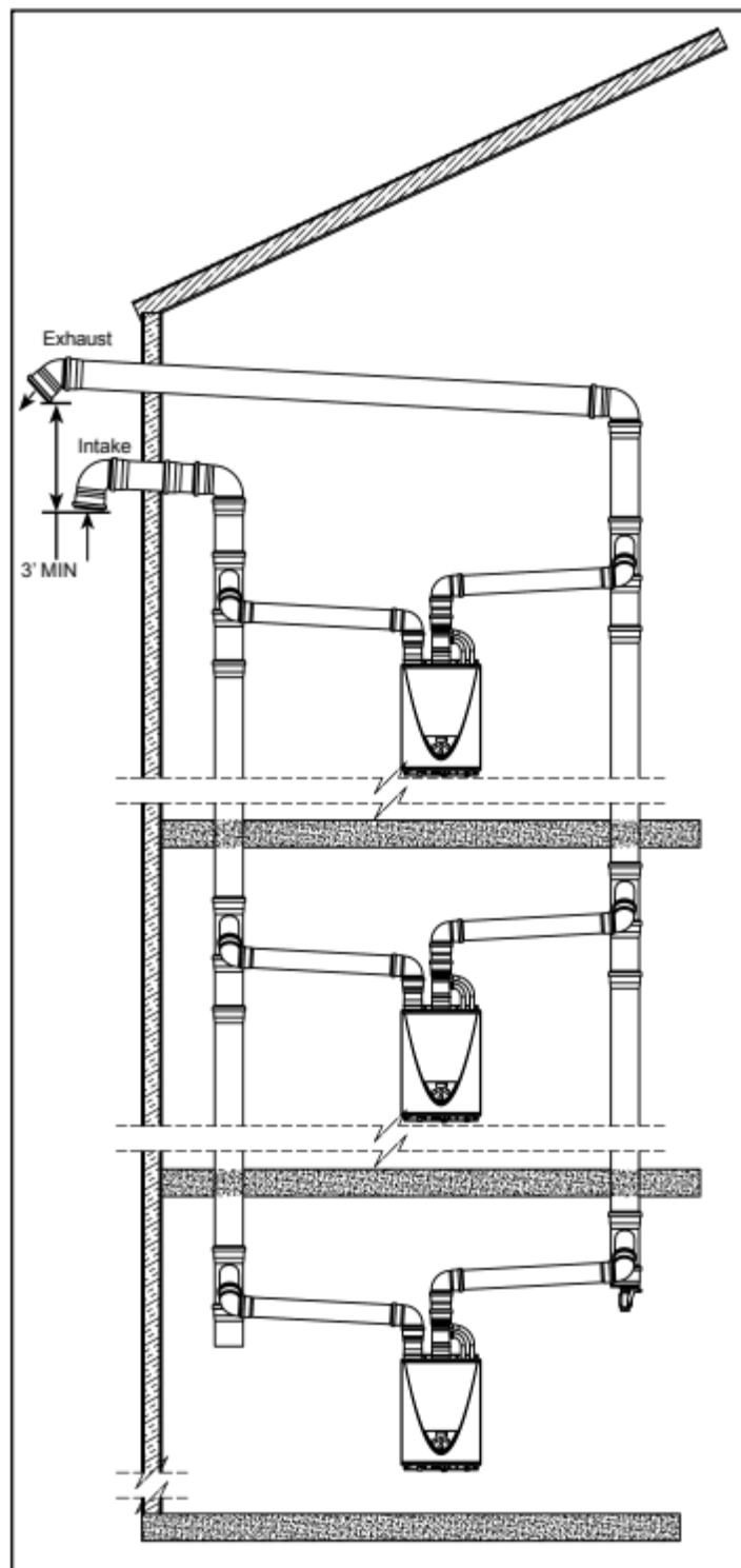
Figure 8. Vertical Through-The-Wall Venting
