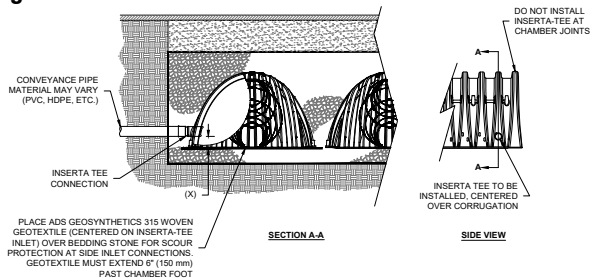
Figure 9 – Inserta Tee Side Detail
