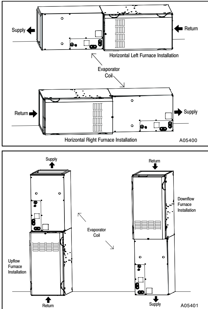
Figure 1 – Correct Orientation of Coil Support on Furnace
