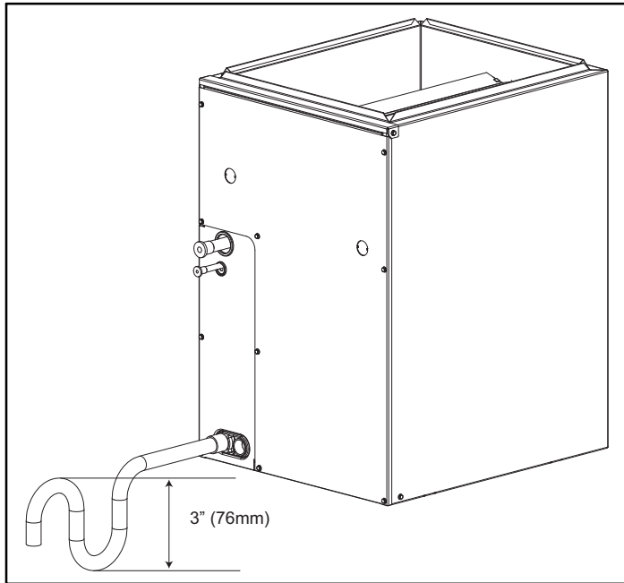
Figure 8 – Condensate Trap
