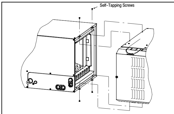
Figure 7 – Horizontal Left Installation
