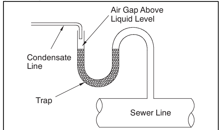
Figure 9 – Condensate Drain to Waste Line
