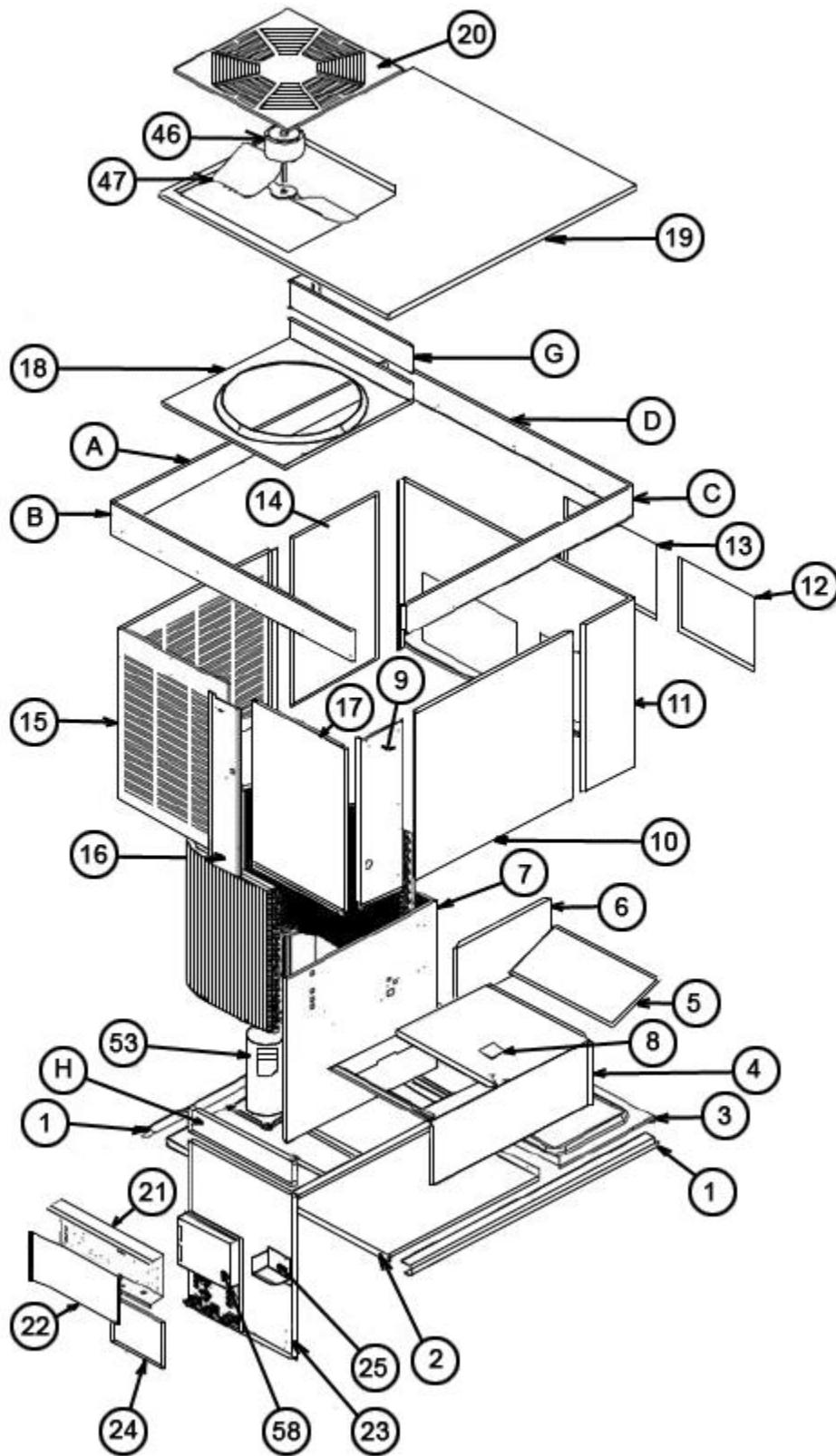
Exploded View
