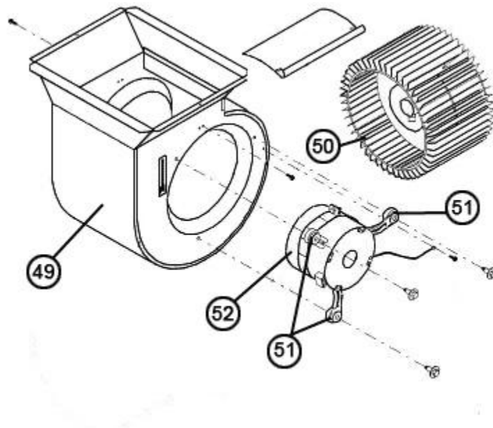
Blower Assembly
