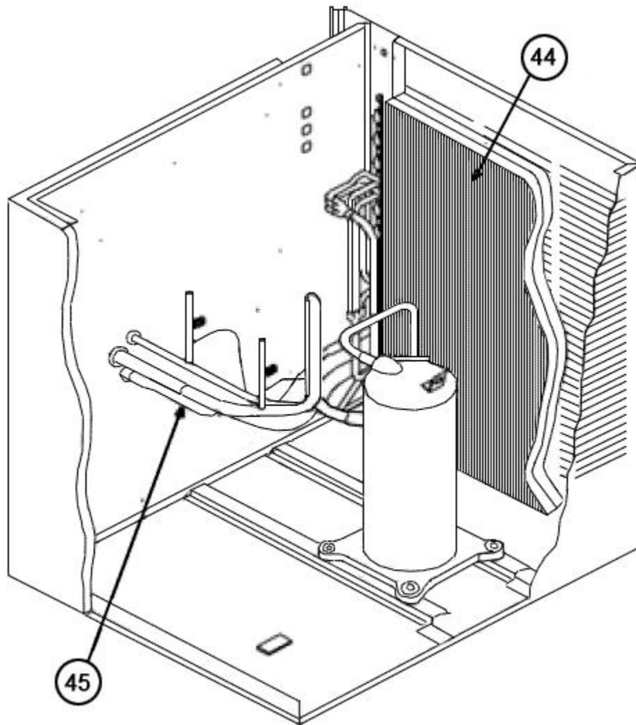
Condenser Coil Assembly
