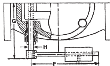
DETAIL LW/LS
