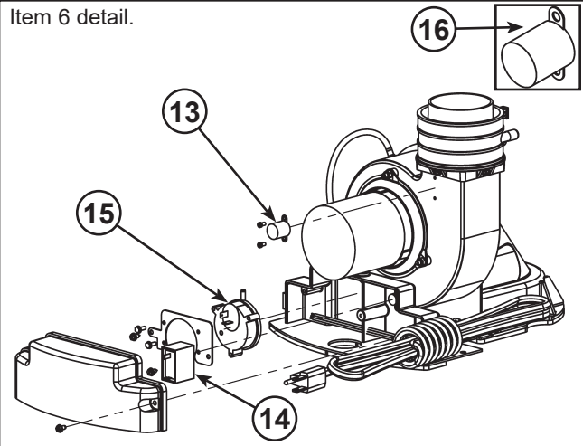
Item 6 detail.
