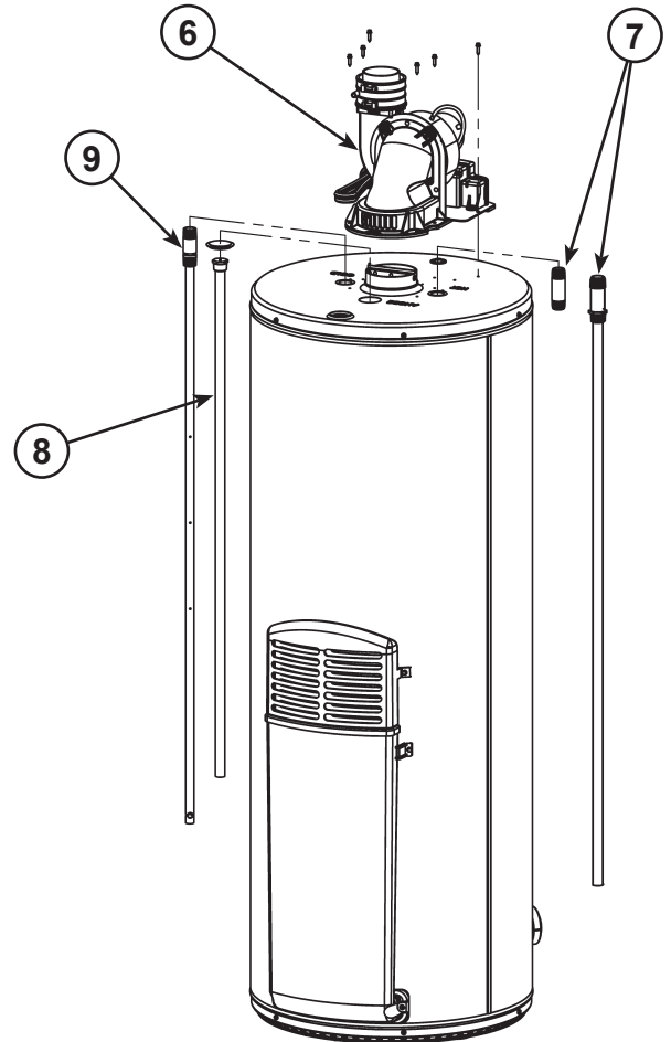
Item 6 detail.
