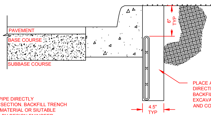
ADVANEDGE INSTALLATION DETAIL (CITY STREET W/ CURB & GUTTER)
