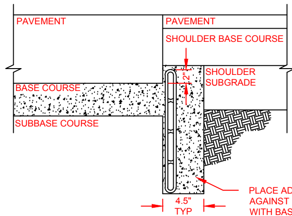
ADVANEDGE INSTALLATION DETAIL (NO CURB & GUTTER)
