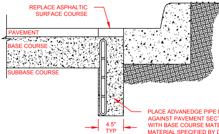
ADVANEDGE INSTALLATION DETAIL (CITY STREET W/ CURB & GUTTER)
