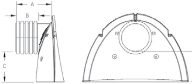
STUB AT TOP OF END CAP FOR PART NUMBERS ENDING WITH "T"
