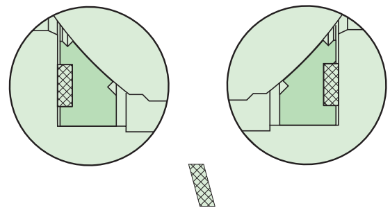
Non-compressed form of the PTFE back seal.
