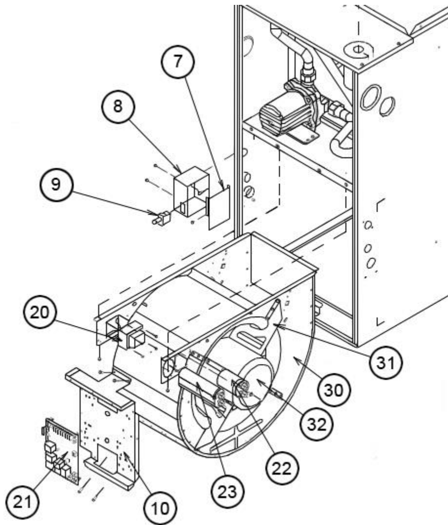
Blower Assembly
