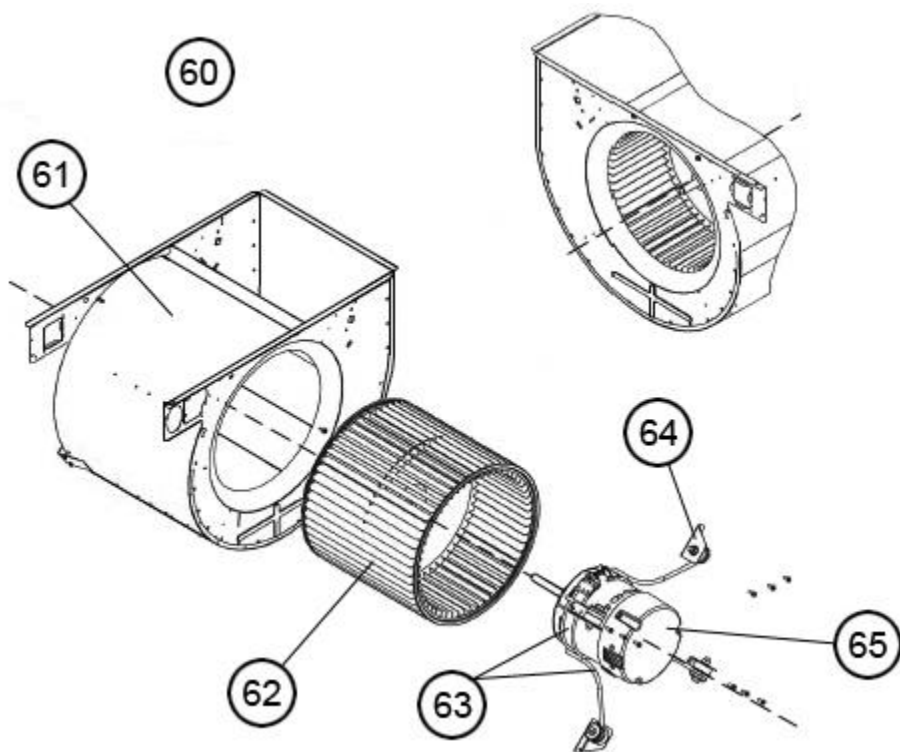
Blower Assembly - ECM Motor
