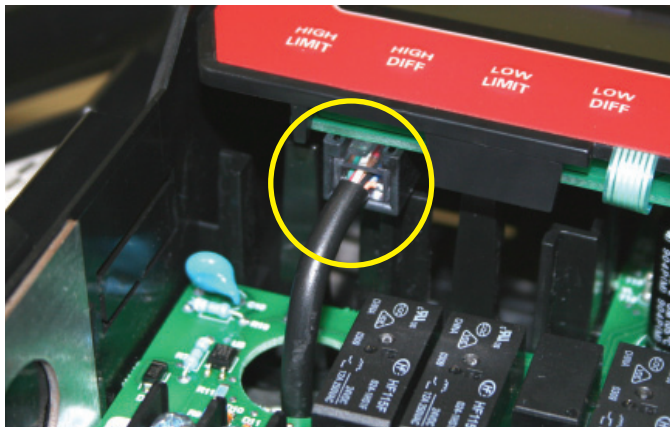
Figure 10 - Temperature Sensor Lead/Receptacle Connection
