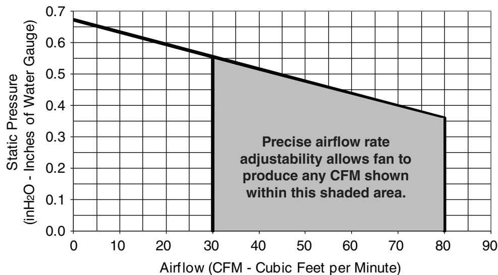
ZN80M - 4" Duct
