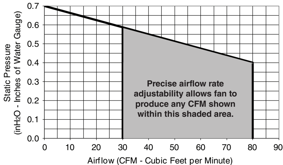
ZN80M - 6" Duct
