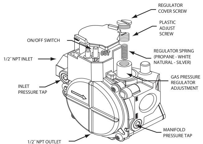
Single-Stage 36G Valve
