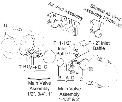
3/4", 1", 1-1/2" FT450
