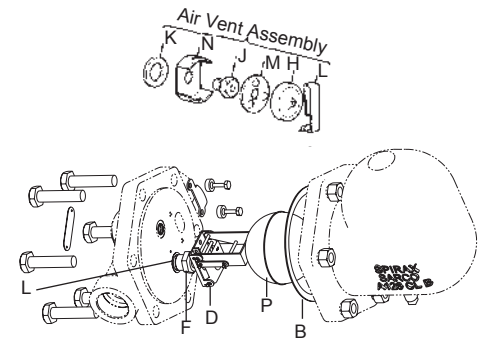
1-1/2" FTI 15 to 200
