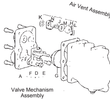
3/4", 1", 1-1/4", 1-1/2" FT-150/200
