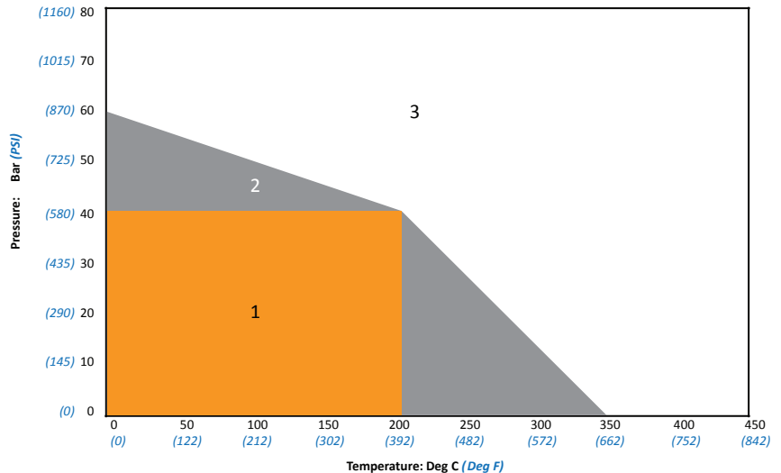
L640W PRESSURE / TEMPERATURE GRAPH
