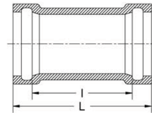
Repair Coupling
