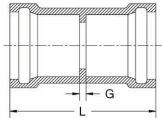
Line Coupling
