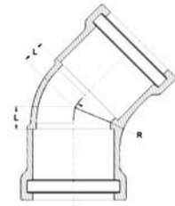
45 Bend
