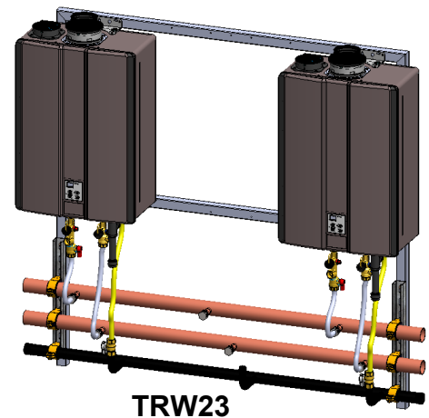
Rinnai Rack Installation
