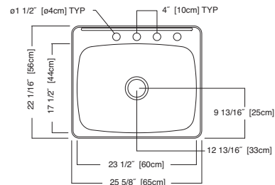
21SB.252284.290 Optional drilling: 4th hole on right
