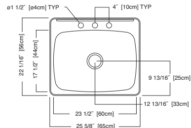
21SB.252283.290 Standard drilling: 3 hole
