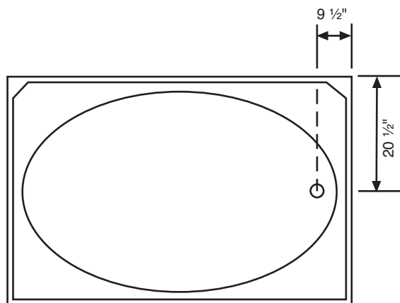
END DRAIN
