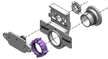
PEXRITE #732 "Exploded"
