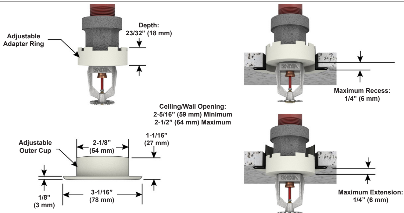
Figure 5: Installation of a Model F-1 Adjustable Escutcheon with 1/2" (12 mm) Total Adjustment.
