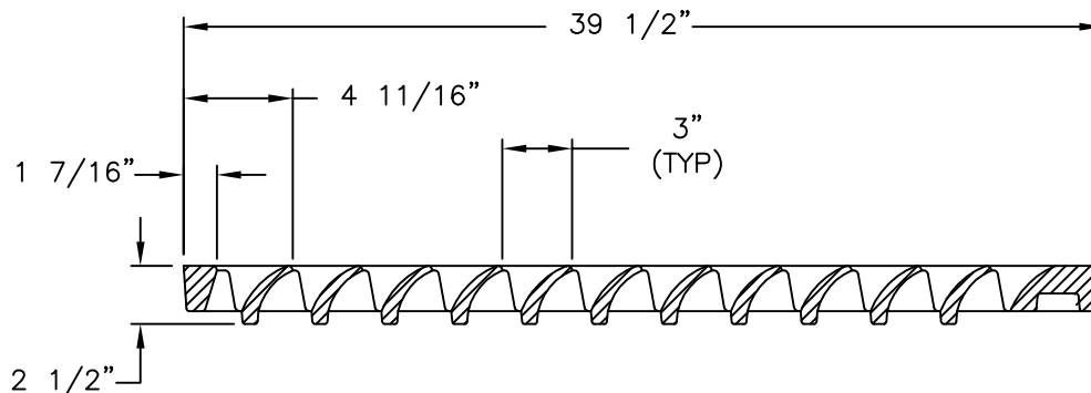
GRATE SECTION
