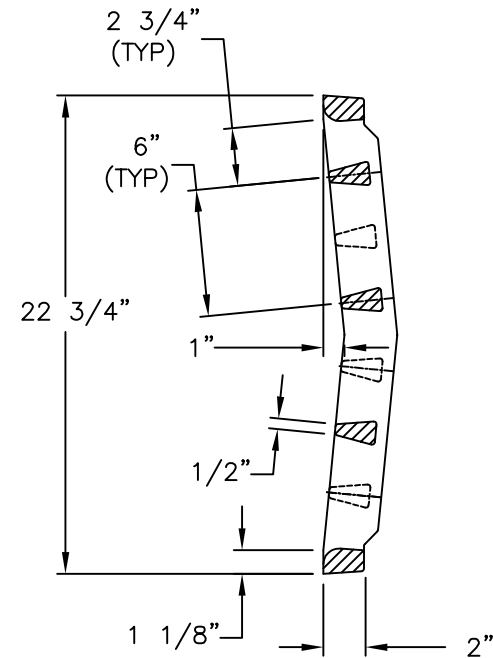
GRATE SECTION
