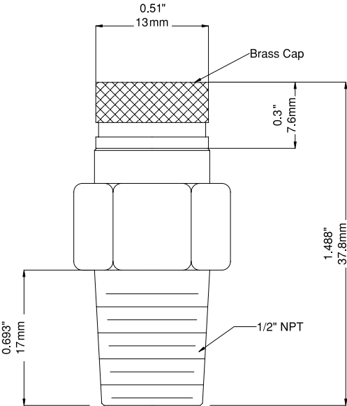
0.5" Test Plug
