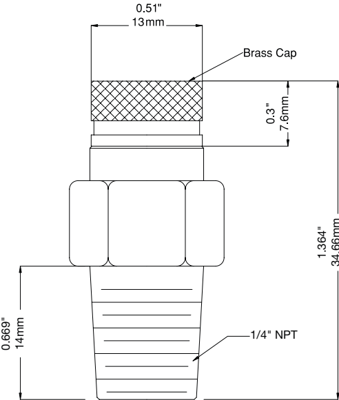
0.25" Test Plug
