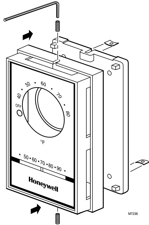
Fig. 4. Locking cover installation.
