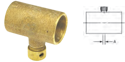
701-D ⚠ Drain Coupling C x C – Cast
