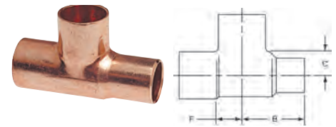
611-2 Fitting Tee C x Ftg x C – Wrot
