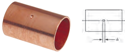
600-DS Coupling with Dimpled Tube Stop C x C – Wrot
