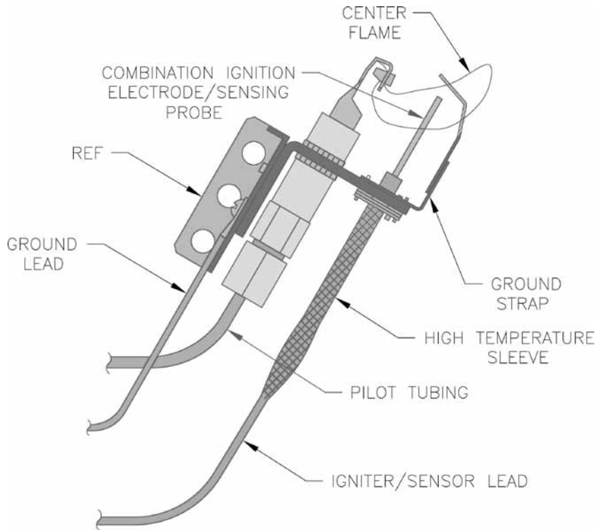
Figure 4: Pilot Burner
