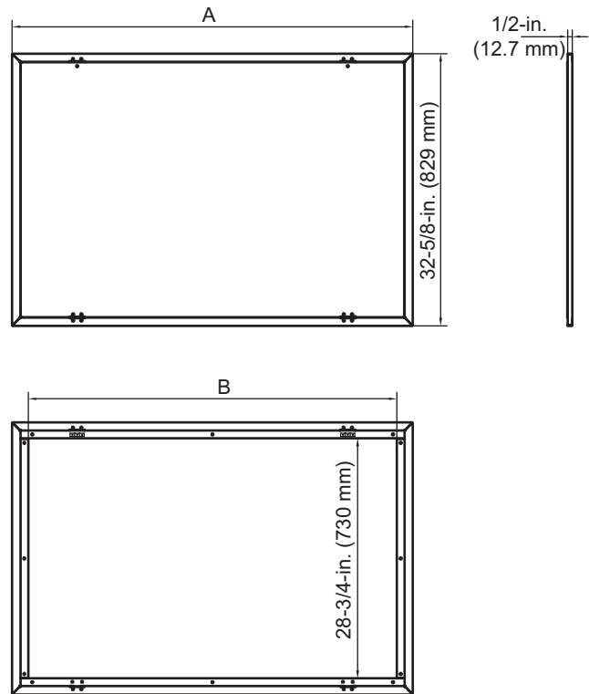
Fig. 1 - Access Panel Dimensions
