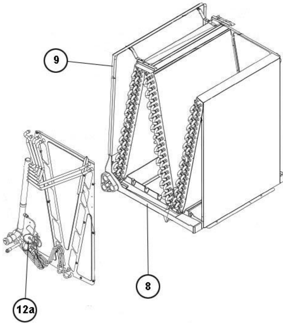
RCHxxxxMTaxUA Coil Assembly
