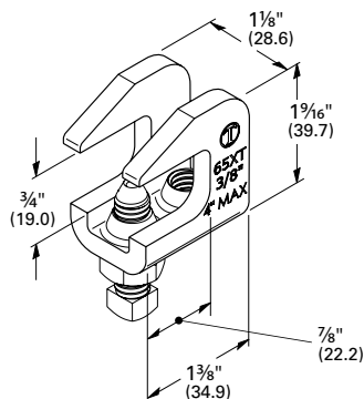
Set Screw Down
