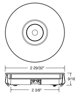
Recessed Mount (USTLR1-3K)
