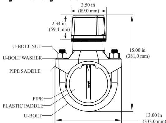
Fig. 7 Mounting Dimensions
