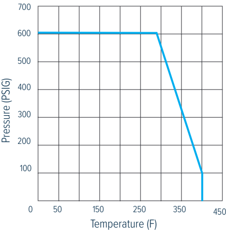
PRESSURE/TEMPERATURE
