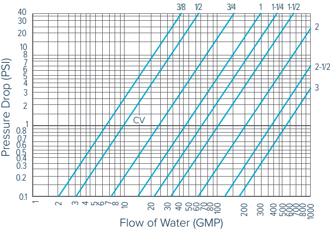
PRESSURE DROP/FLOW OF WATER
