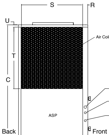
Left Return Left View - Air Coil Opening
