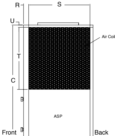
Right Return Right View - Air Coil Opening
