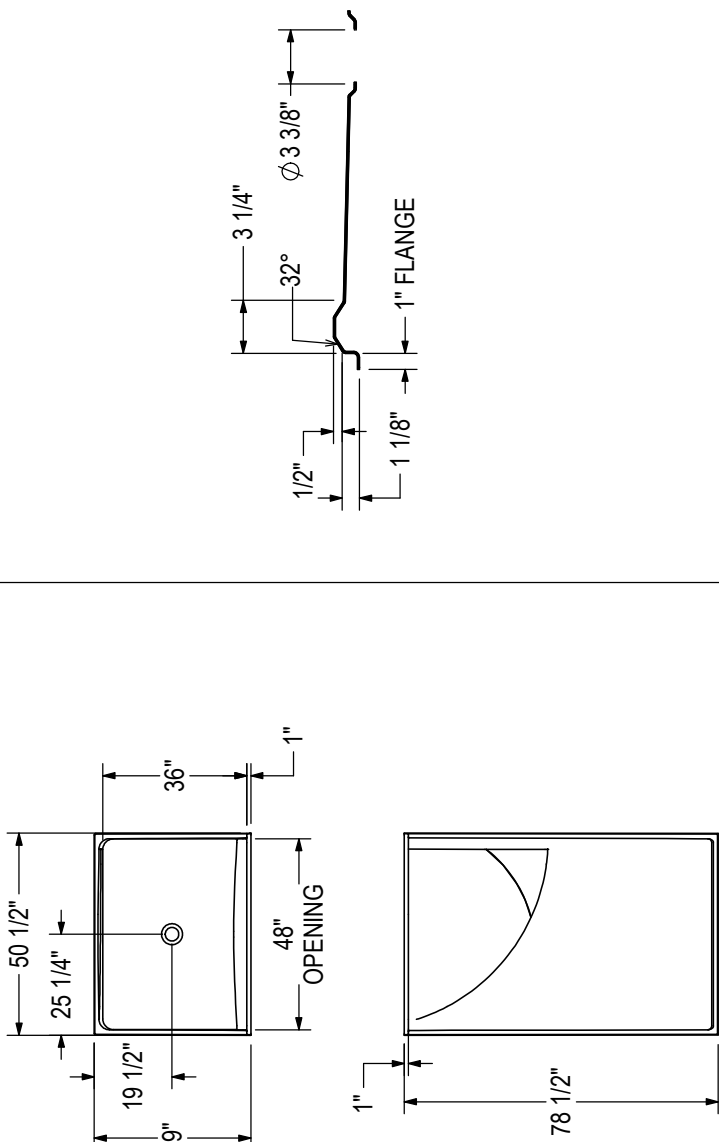
THRESHOLD DETAIL
