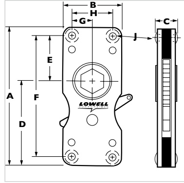
700 Series Clutches
