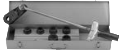
Model 513
