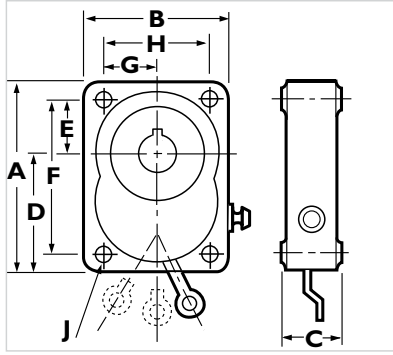
70 Series Clutches
