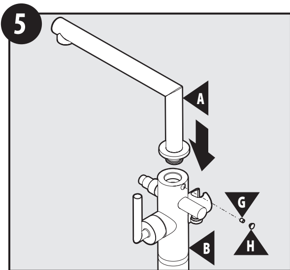
Install Spout (A) onto Faucet Body (B). Secure with Set Screw (G) and Plug Button (H).
