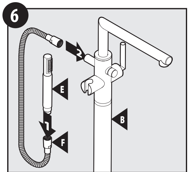
1. Install Hose (F) and Hand Shower (E). 2. Install other end of Hose (F) onto Faucet Body (B).
