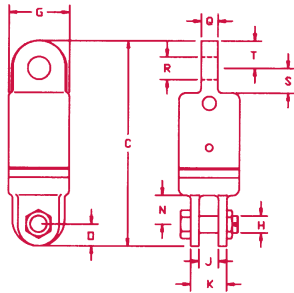
S-4 Eye & Jaw
