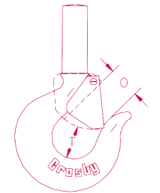
Shank Hook dimension with PL Latch Assembled
