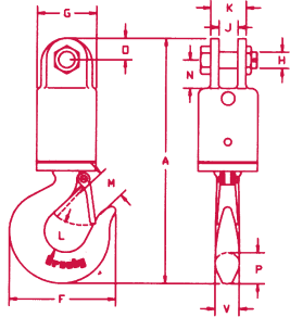
S-1 Jaw & Hook
