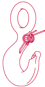
Figure 5: IMPORTANT — Instructions for Assembling S-4320 Latch on Crosby 320N Hooks
