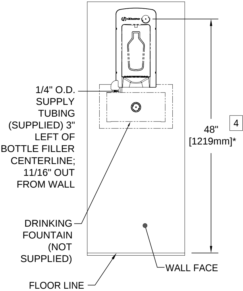
TYPICAL DRINKING FOUNTAIN INSTALLATION
