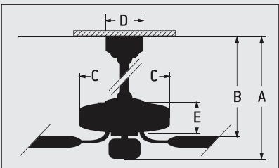
A: 6" DR - 15.51" C: 6.31" E: 9.59" B: 6" DR - 13.23" D: 5.11" DR = Downrod
