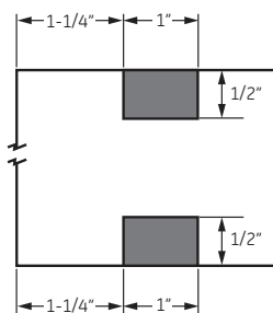
Top/Bottom Hinge Clearance Router 1/8" Deep
