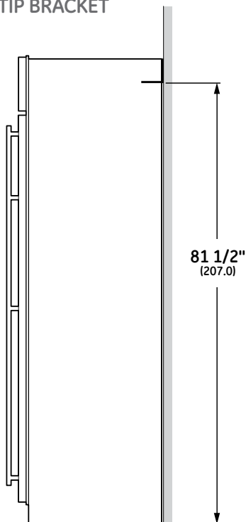
SIDE VIEW INSTALLED WITH ANTI-TIP BRACKET
