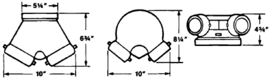
MODEL 5710 - 5715
